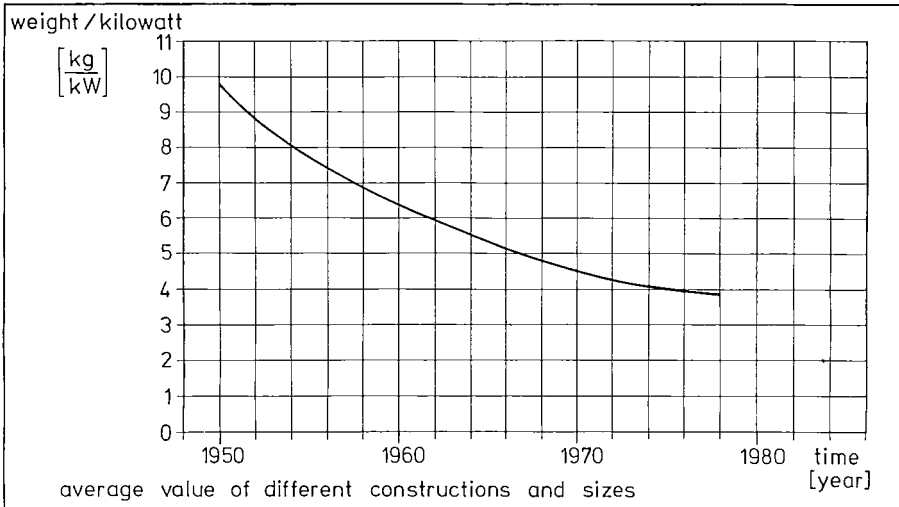
Fig.3. Reduction of the weight/kilowatt value of submersible motors from 1950 until 1978
