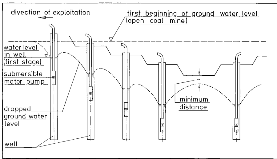
Fig.4. Section through an open coal mine
