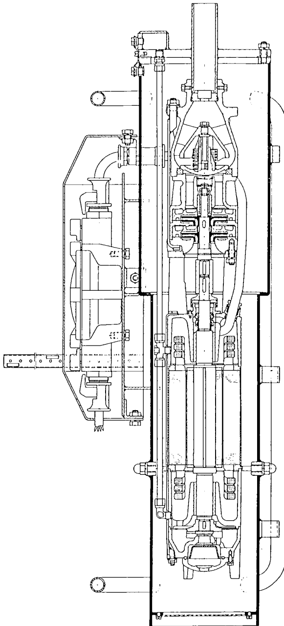
Fig. 9 - cut through a explosion-proof submersible unit, type UPD 62/6 + sDF 0203
