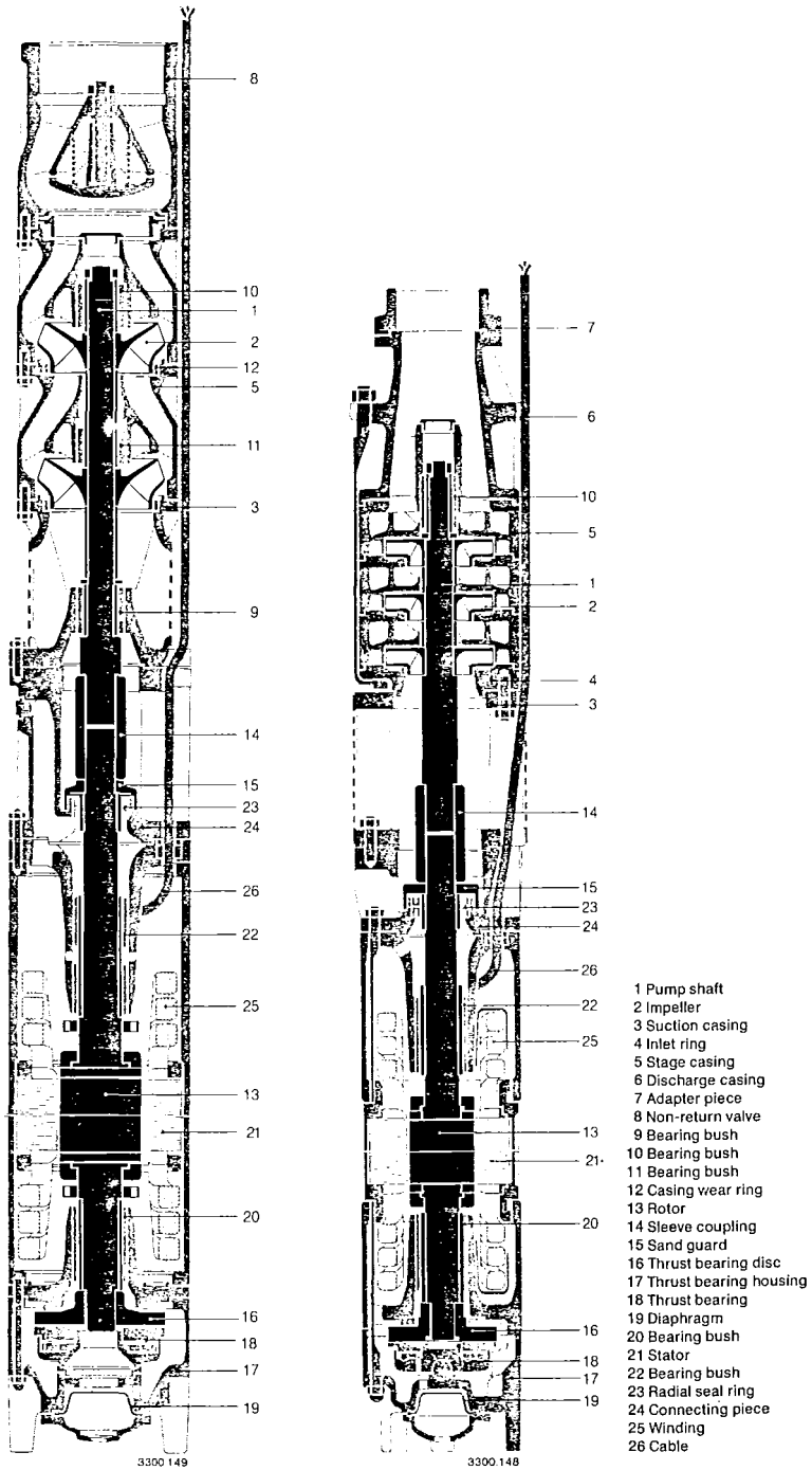
Fig. 1: Submersible motor pump
