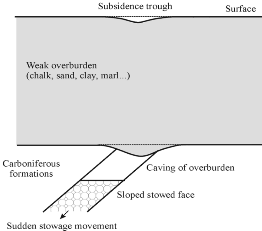
Figure 4 Subsidence restoration due to the untamping of a stowed sloped face
