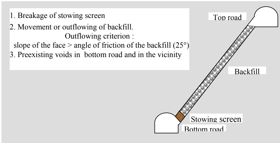
Figure 2 The three simultaneous conditions for the backfill outflow of a stowed sloped face
