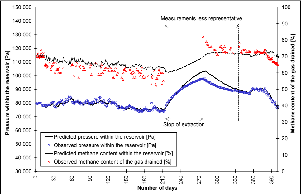
Figure 6 Predicted and observed values of the pressure and methane content within the reservoir
