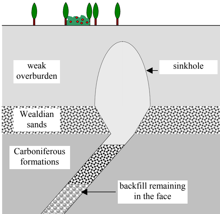
Figure 3 Sinkhole mechanism initiated by the backfill outflow of the stowed sloped face with the presence of Wealdian sands in the overburden (North and Pas-de-Calais coal basin)
