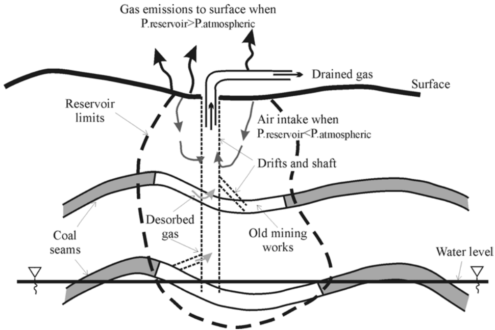
Figure 5 Schematic representation of a mine gas reservoir
