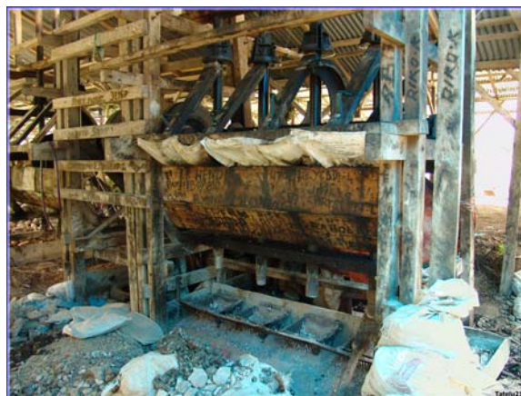
Figure 9. Atop each rod, or stamp, is an eccentric wheel that raises then drops the stamp to crush the ore in bins beneath.
