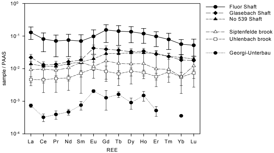
Fig. 1. Rare earth element (REE) patterns for the Straßberg/Harz and Georgi-Unterbau mine and surface waters normalized to Post Archean Australian Shales (PAAS). Filled symbols: mine waters; open symbols: surface waters. Error bars for 25 % and 75 % percentiles.
