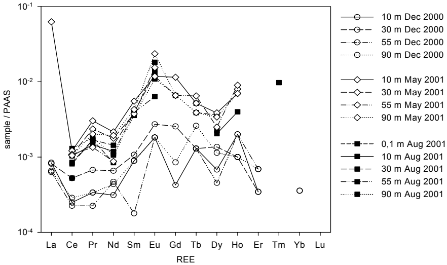
Fig. 2. Depths depended rare earth element (REE) patterns for the Georgi-Unterbau mine waters normalized to Post Archean Australian Shales (PAAS). Data of three sampling periods in December 2000, May, and August 2001, respectively.
