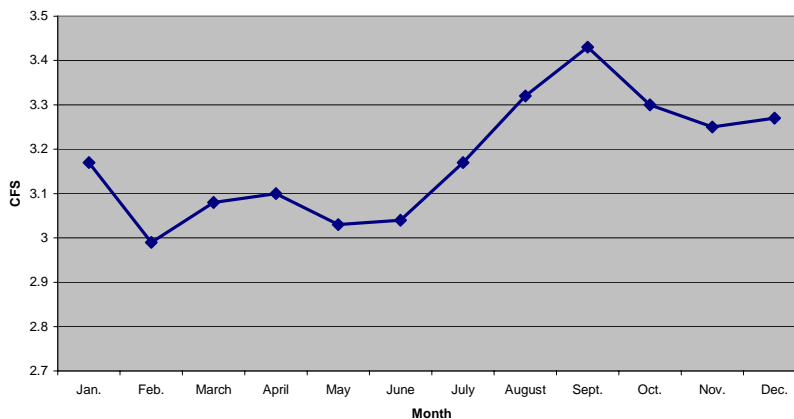
Figure 15 – LMDT Mean Monthly Discharge – January 1998 – July 2004
