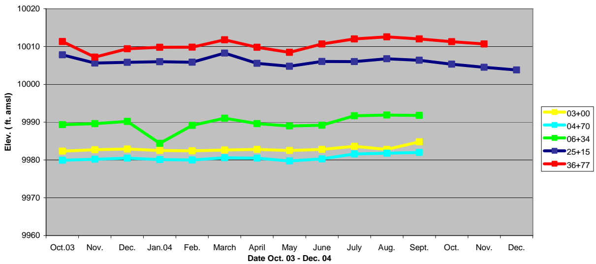
Figure 13 - Water Level Elevations, Tunnel Wells Below Pendery Fault - Oct. 2003 - Dec. 2004
