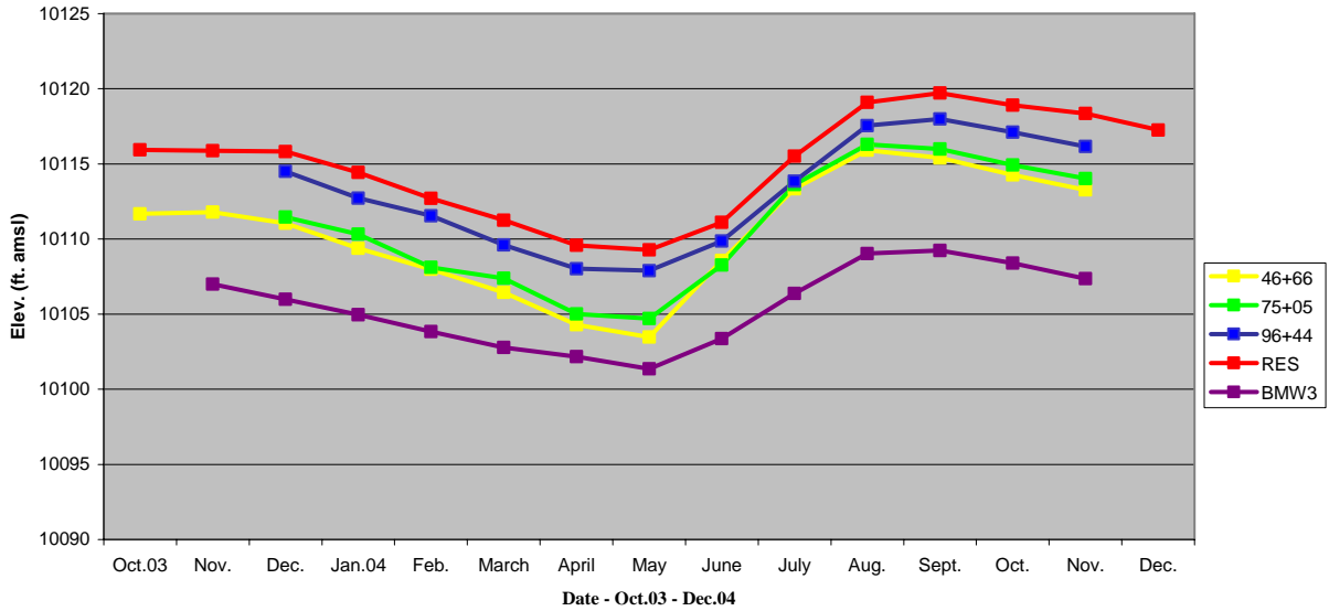
Figure 12 - Water Level Elevations - Tunnel Wells Above Pendery Fault, RES & BMW-3 - Oct. 2003 - Dec. 2004
