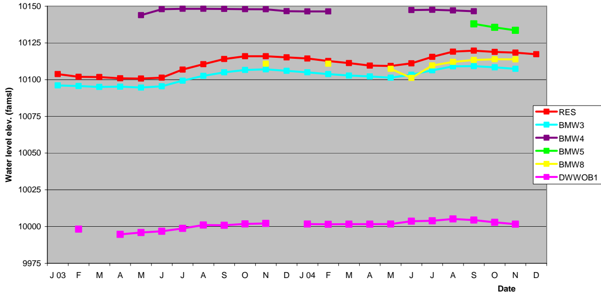
Figure 8 - Water Level Elevations - RES and Bedrock Wells in Vicinity of LMDT
