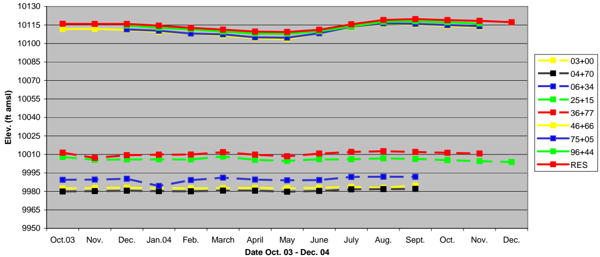
Figure 11 - Water Level Elevations - All Tunnel Wells & RES (Pendery Fault @ 4000 ft From LMDT)
