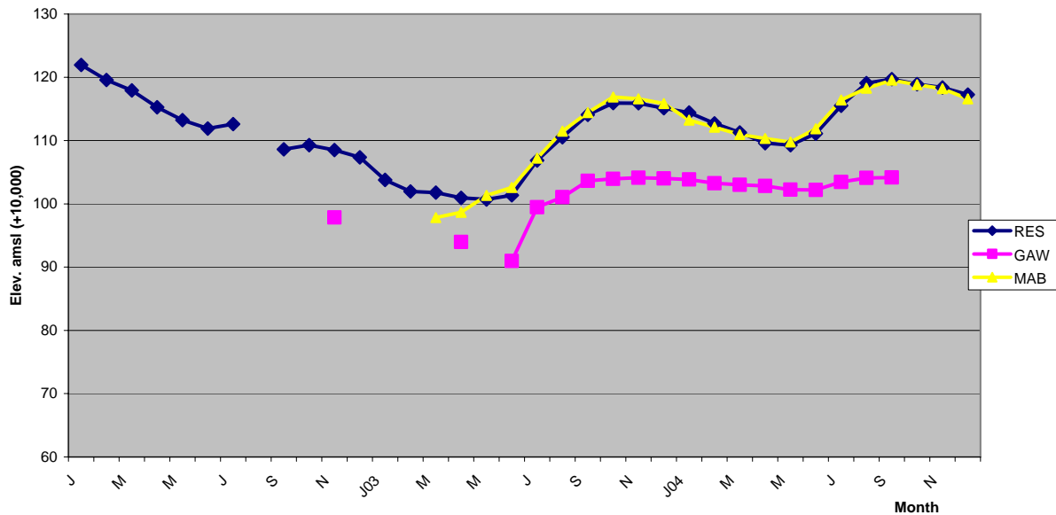
Figure 10 - Water Level Elevations in the RES, Gaw Shaft & Mab Shaft - Jan. 2002 - Dec. 2004
