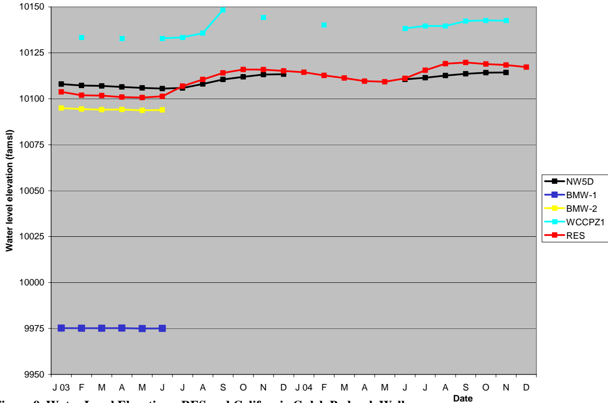
Figure 9 Water Level Elevations, RES and California Gulch Bedrock Wells
