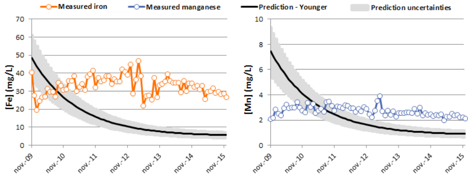
Figure 3 – Iron and manganese evolution at the pumping station of La Houve.
